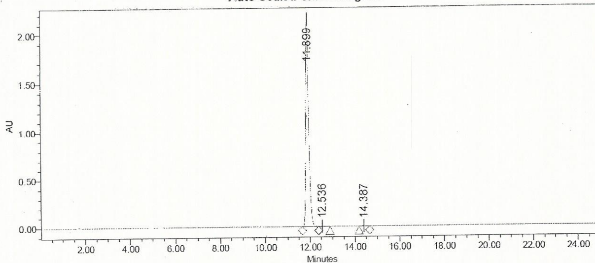
Auto-Scaled Chromatogram
